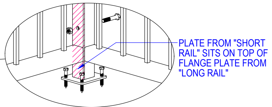
DETAIL B SCALE 1 : 8
